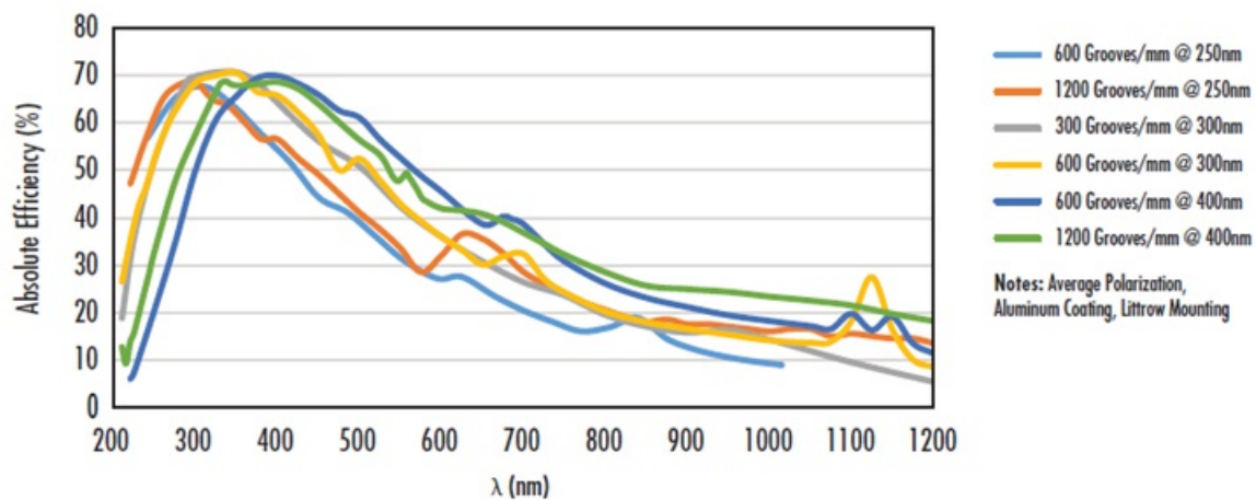
Typical Efficiency Curves for Ruled Gratings Optimized (Blaze) Wavelengths from 250 - 400nm
