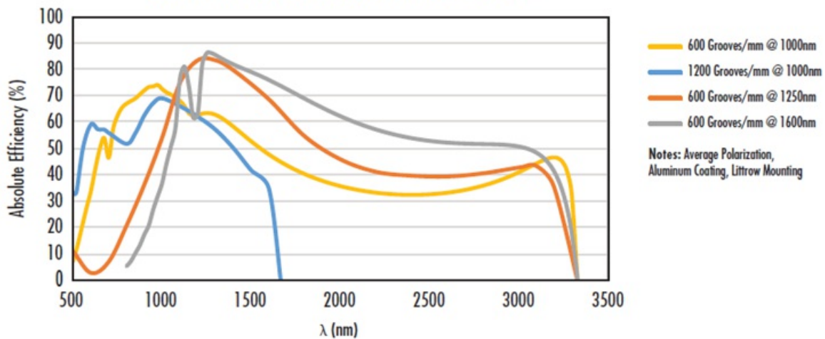
Typical Efficiency Curves for Ruled Gratings Optimized (Blaze) Wavelengths from 1000 - 1600nm
