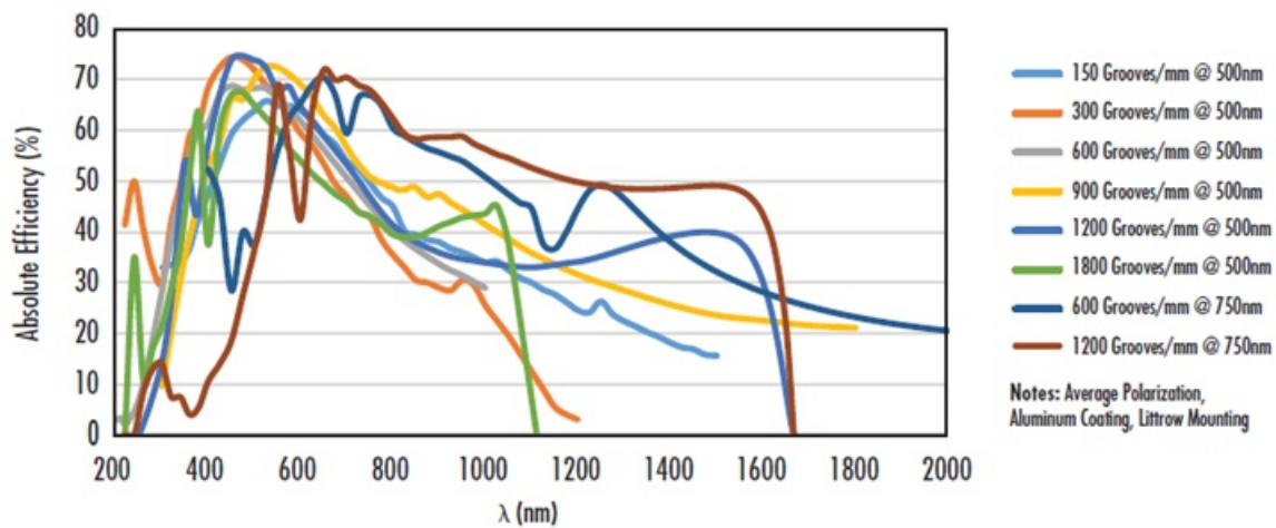
Typical Efficiency Curves for Ruled Gratings Optimized (Blaze) Wavelengths from 500 - 750nm
