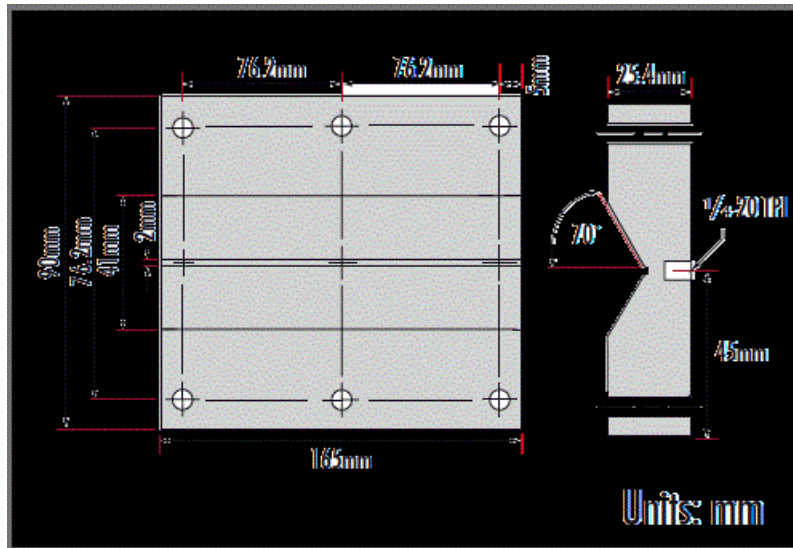
V-Block Base
