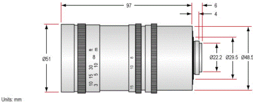
Manual Zoom Video Lens #53-152
