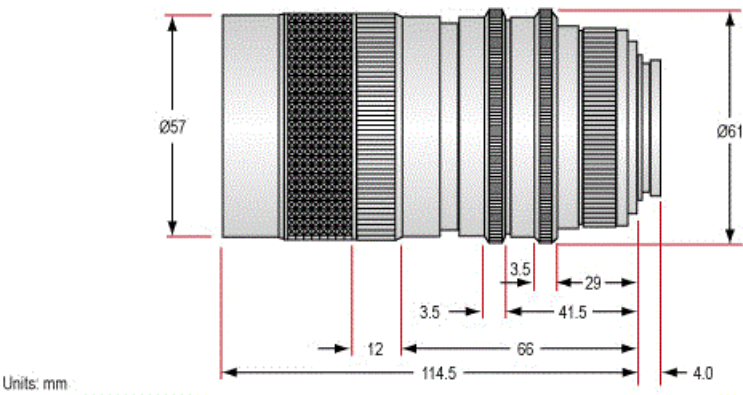
Manual Zoom Video Lens #53-153
