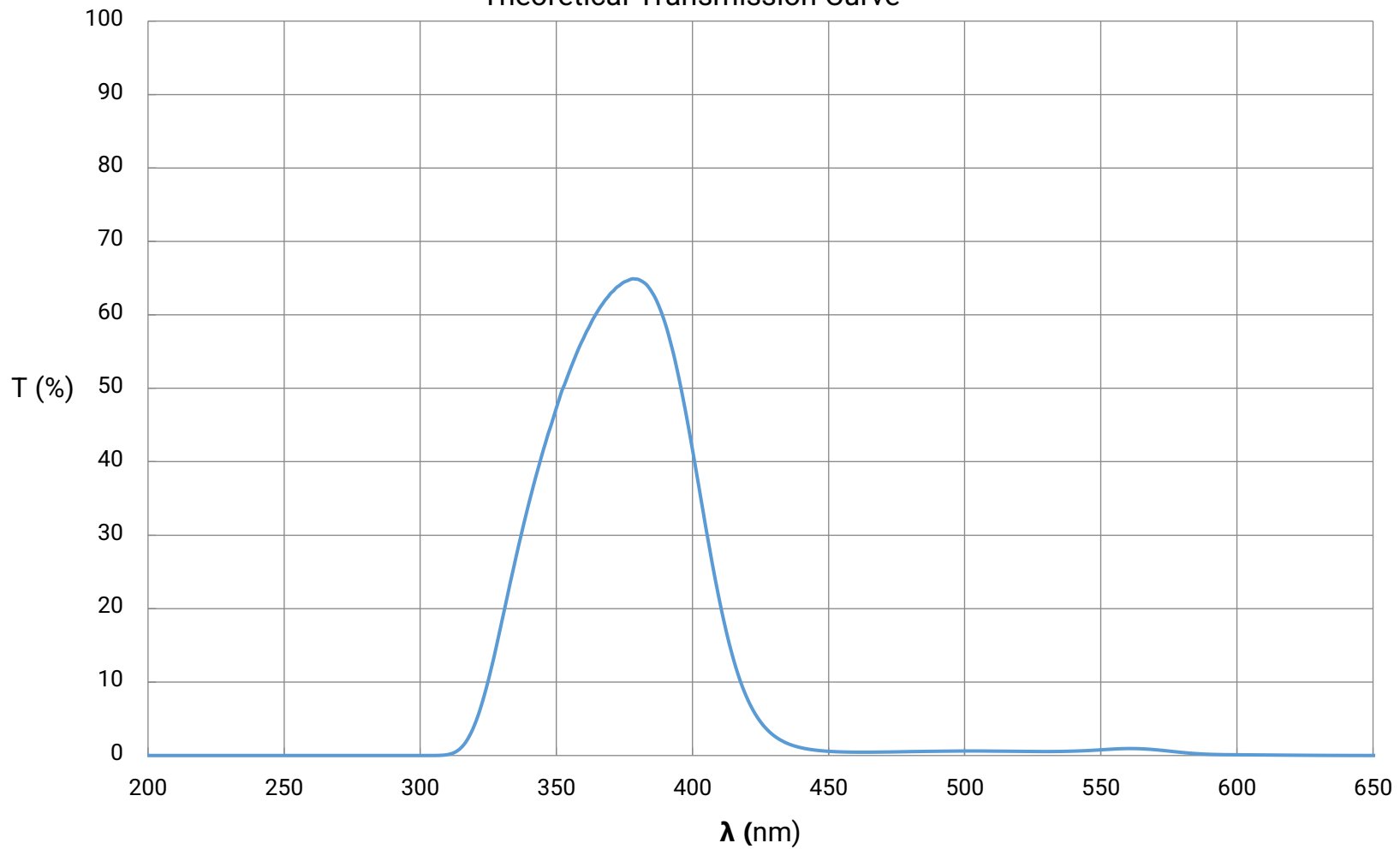
Astronomy Bandpass Filter, UV Theoretical Transmission Curve
