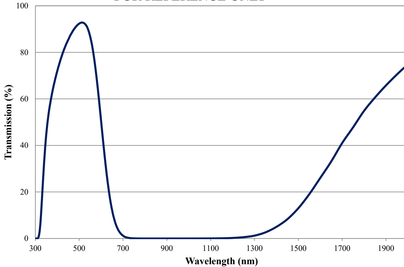
BG42 Colored Glass Filter Internal Transmittance 1mm Thickness FOR REFERENCE ONLY
